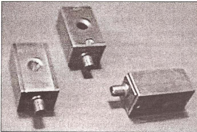
Fig. 8. The 2 GHz central frequency and 1.5 GHz bandwidth near infrared light deflectors based on resonant AO effect.
