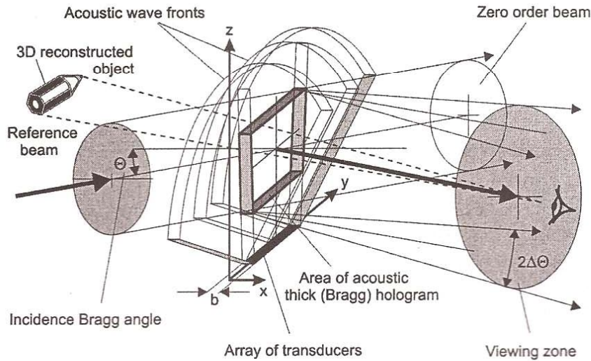
Fig. 9. Architecture of holographic display based on AO interaction.
