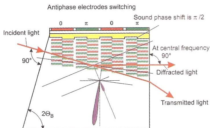
Fig. 2. Light interaction with one-petal sound beam generated by anti-phase array with additional phase shift.
