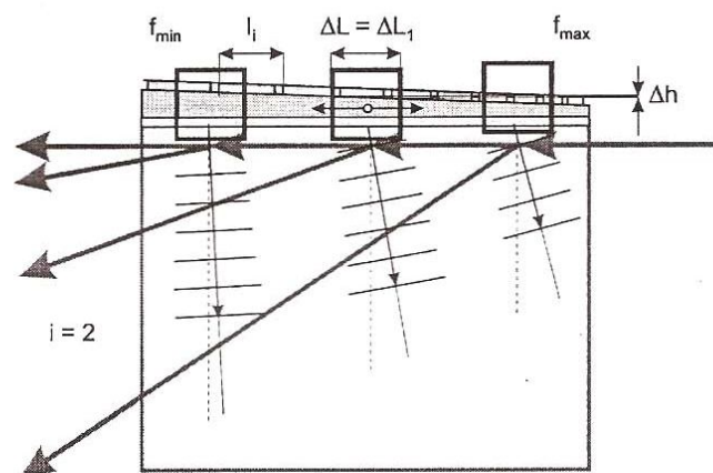
Fig. 4. Moving window multielement transducer system for Bragg angle and resonant frequency automatic tuning.
