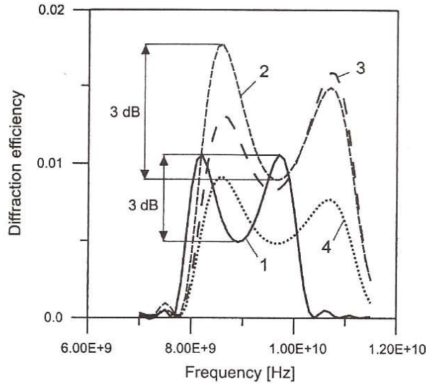
Fig. 5. Diffraction efficiency frequency dependences when different types of multielement transducers are used (curve 1 – in-phase system with constant step of array; curves 2, 3 – variable step arrays with exponential and linear electric power distribution; curve 4 – variable step and constant electrical power).
