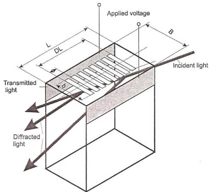
Fig. 3. AO cell with electronically tunable multielement array periodicity.
