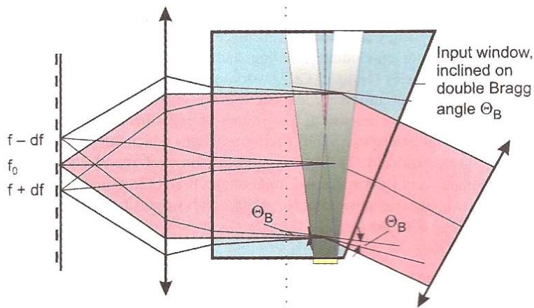
Fig. 1. AO interaction geometry with sound beam generated by anti-phased multielement transducer.
