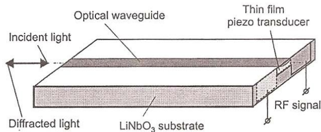
Fig. 7. Integrated collinear AO tunable mirror.
